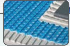
Actual image of ProVa-Lay. Dimensions - 1 panel: 2' x 3.2' (6.5 sq. ft.) 30 panels/carton (195 sq. ft.)
